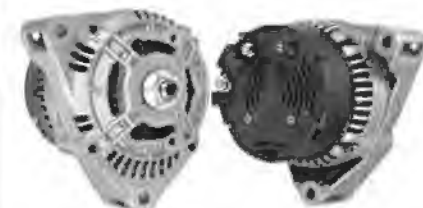
Bosch Type, 12V/90A USED ON: AUDI AND VOLKSWAGEN 1986-92 CARGO#: 111079 HC-Parts: CA320IR OEM#: 0-123-335-001 WOODAUTO: ALT10113 WAI#: 1-1388-00BO
