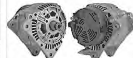
Bosch Type, 12V/90A USED ON: VOLKSWAGEN BEETLE 2.0L 1998 CARGO#: 111820 HC-Parts: CA1240IR LESTER: 13903 OEM#: 0-123-320-034 WOODAUTO: ALT10038 WAI#: 1-1539-00BO
