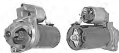
Bosch Type, 12V/2.2KW/9T
